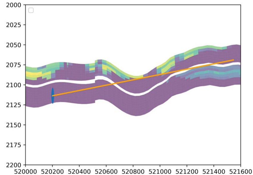
Neural network assisted: Geosteering
