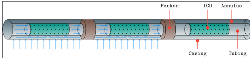
Packer and ICD optimization
